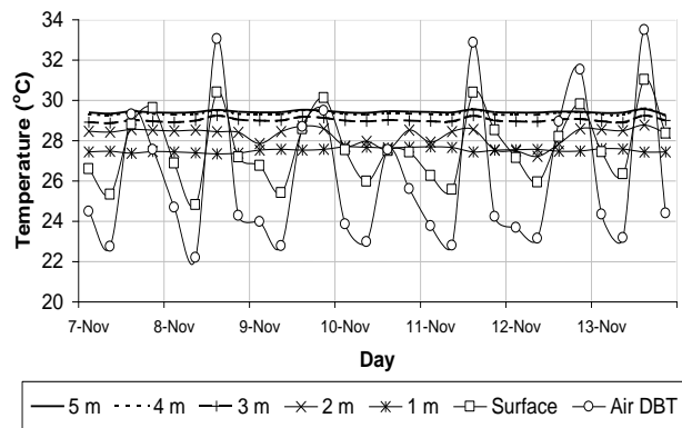
Figure-4. Temperature patterns in week 4
