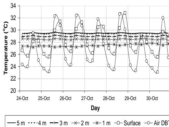
Figure-1. Temperature patterns in week 2
