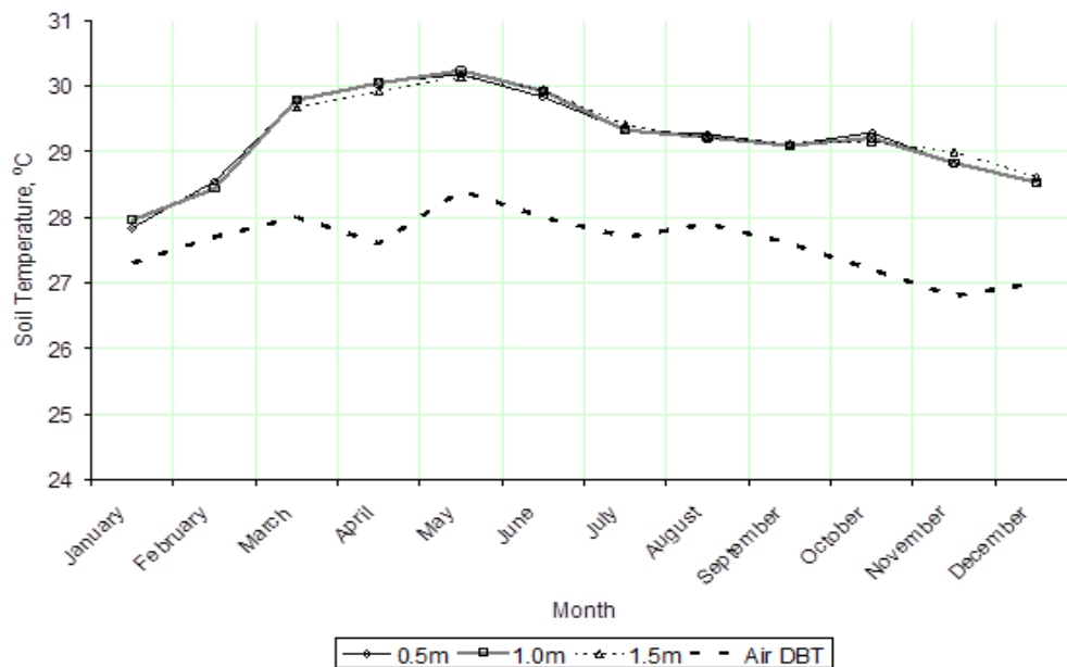
Figure-5. Average air temperature and soil temperature at 0.5m, 1.0m and 1.5m depths underground
