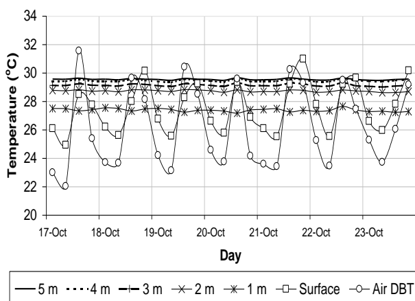
Figure-2. Temperature patterns in week 1
