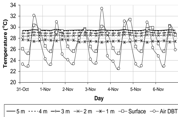
Figure-3. Temperature patterns in week 3
